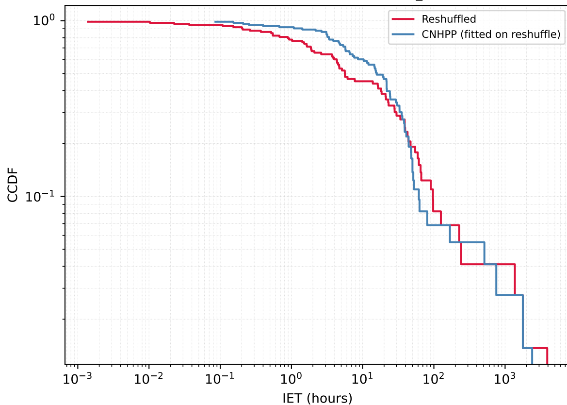
User 438601269 - Reshuffled vs CNHPP A_{\text{fit}}=0.6677
